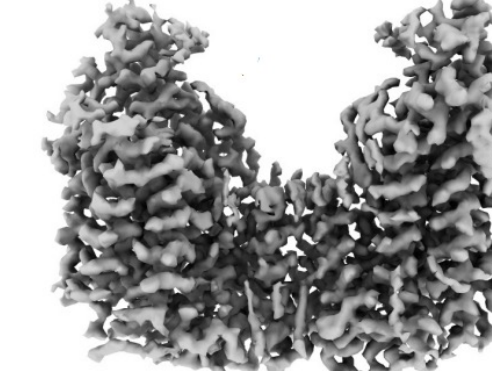
NKCC1 TM domain
